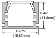
MOSR-CHAN-SLV-6.5 Anodized aluminum extrusion available in 6.5' length
