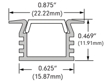
EDIN-CHAN-SLV-6.5 Anodized aluminum extrusion available in 6.5' length
